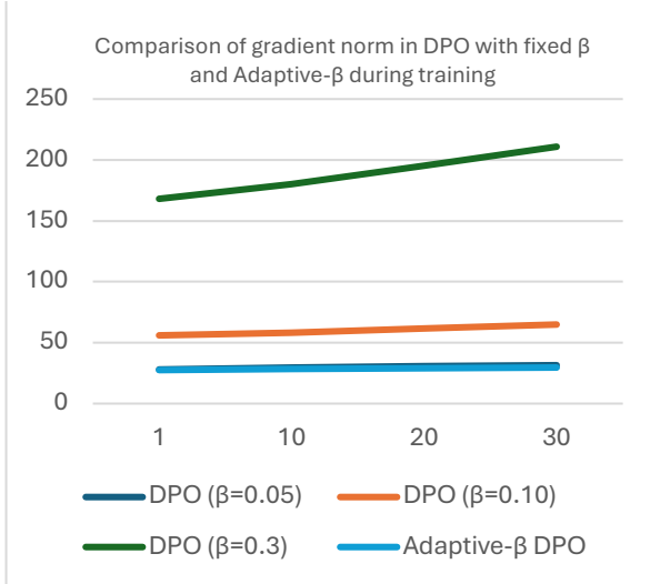
Figure 2. Comparison of DPO with fixed and adaptive \beta values
