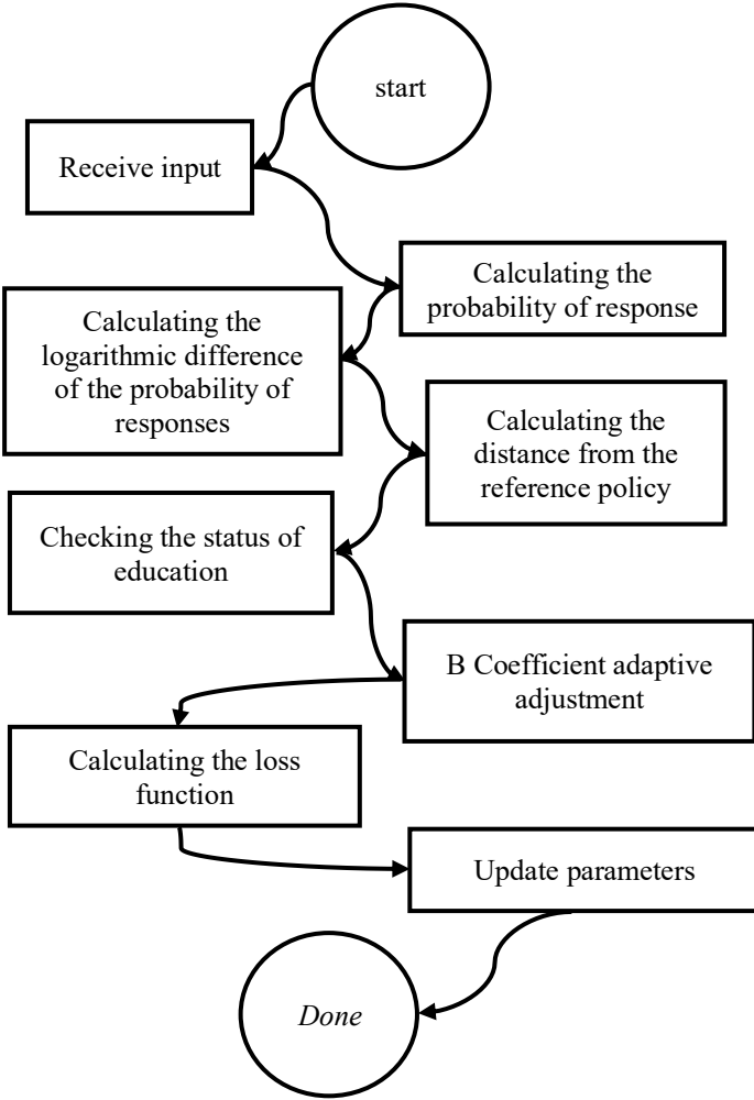
FIGURE 1. ILLUSTRATES THE OVERALL WORKFLOW OF THE PROPOSED ADAPTIVE- \beta DPO ALGORITHM
